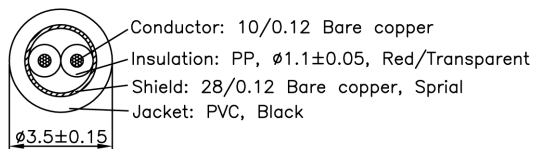
Cable construction
