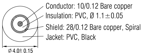
Cable Construction
