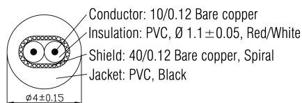
Cable Construction
