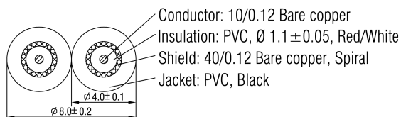
Cable Construction
